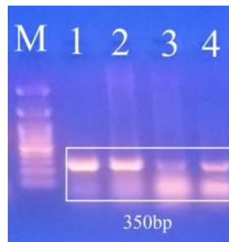
Figure 5- The results of RT-PCR test in 1% agarose gel including samples infected with Potyvirus from Dieffenbachia sp. Plants.
